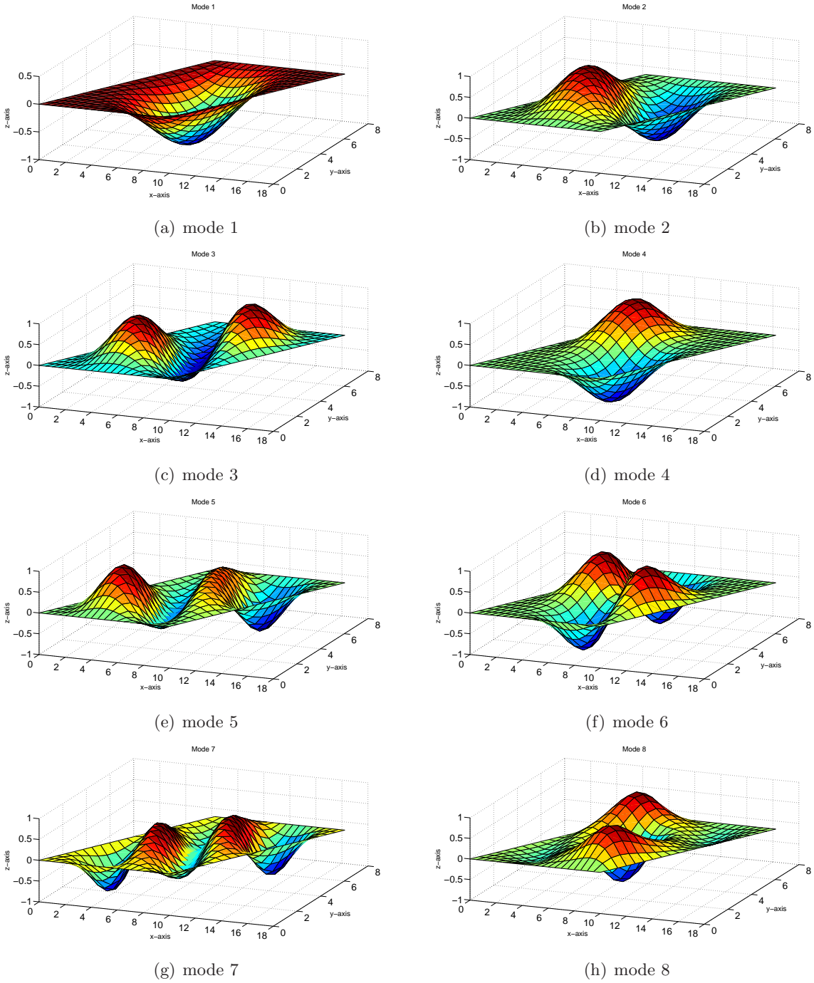
Figure 20: First eight mode shapes for a clamped Al/ZrO 2 skew plate with a/h = 10 , gradient index n = 0.5 and \psi = 45^\circ .
