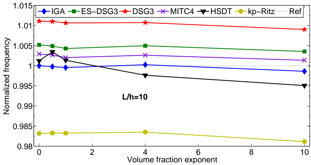
Figure 14: The normalized first frequency \bar{\omega} = \omega/\omega_{\text{ref}} versus volume fraction exponents for SSSS Al/Al 2 O 3 FGM plate with a/h = 10 . The frequency is normalized with the analytical solution.
