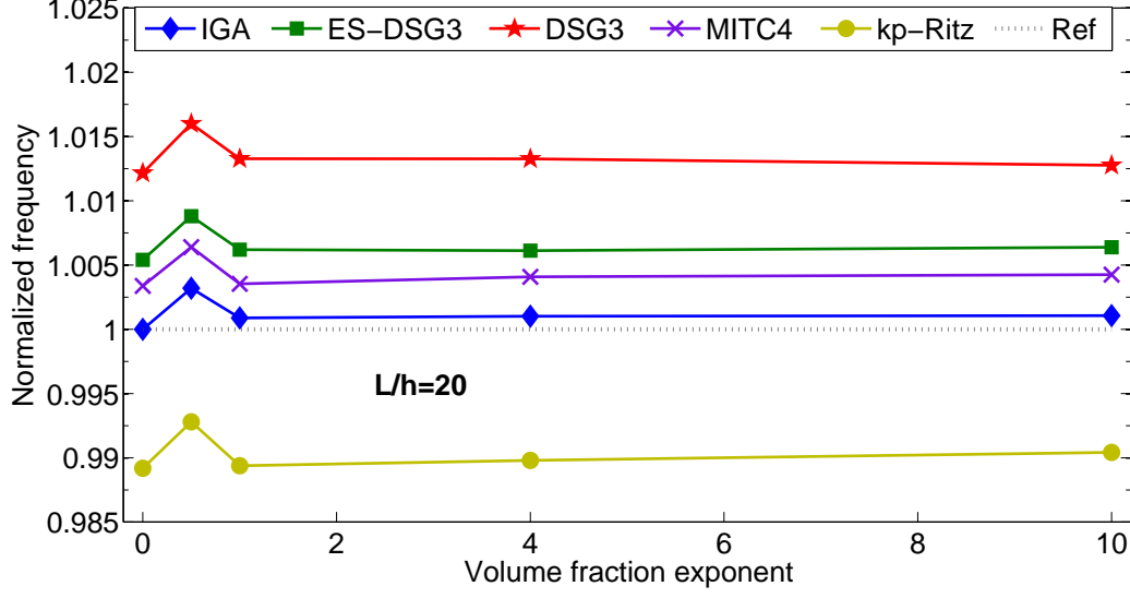
Figure 15: The normalized first frequency \bar{\omega} = \omega/\omega_{\text{ref}} versus volume fraction exponents for SSSS Al/Al 2 O 3 FGM plate with a/h = 20 . The frequency is normalized with the analytical solution.
