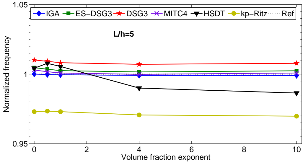
Figure 13: The normalized first frequency \bar{\omega} = \omega/\omega_{\text{ref}} versus volume fraction exponents for SSSS Al/Al 2 O 3 FGM plate with a/h = 5 . The frequency is normalized with the analytical solution.
