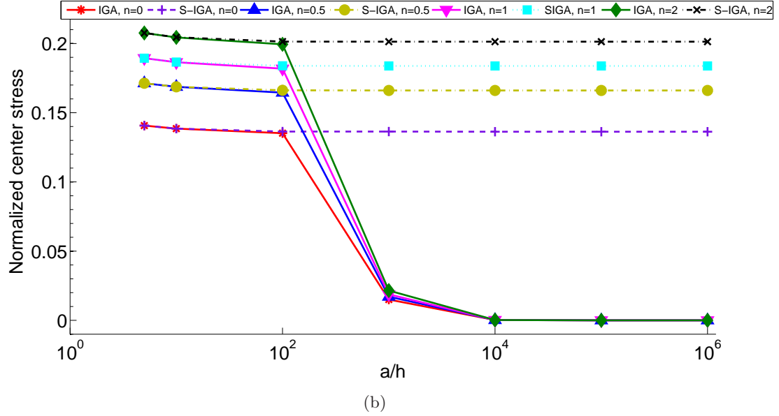
Figure 4: The normalized center deflection, \bar{w}_c and the normalized axial stress \bar{\sigma}_{xx} as a function of a/h for a clamped Al/Zr0.2-1 FGM square plate subjected to a uniform load, p : (a) normalized center deflection and (b) normalized center stress.
